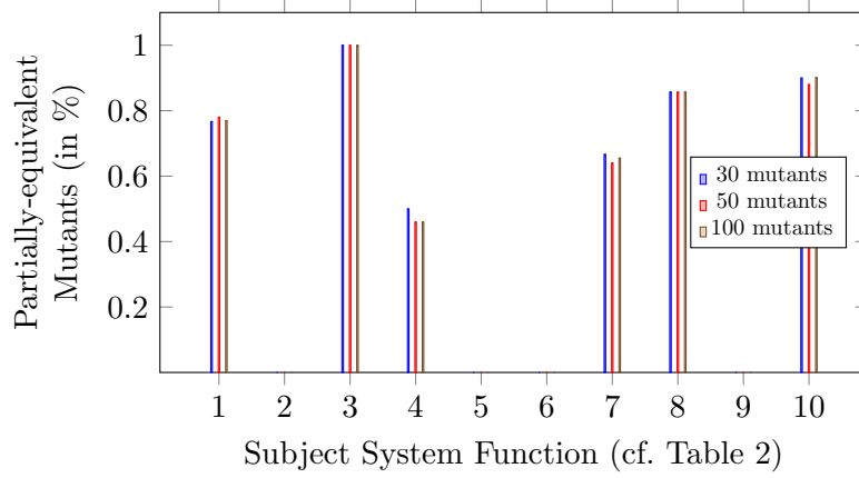
(a) Percentage of Partially-equivalent Mutants
