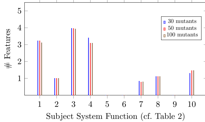
(c) # Features Necessary to Detect a Mutant
