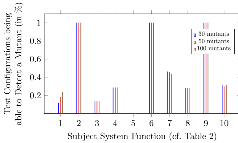
(b) Percentage of Test Configurations being able to Detect a Mutant
