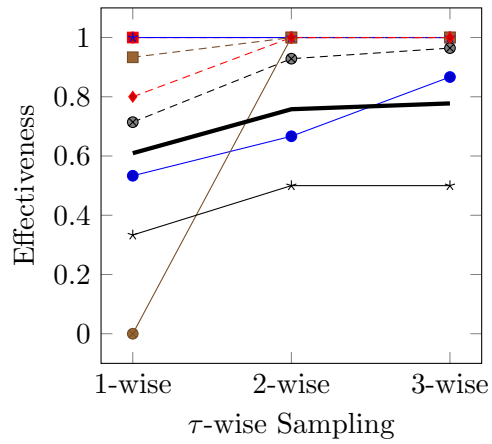
(b) Effectiveness of Samples
