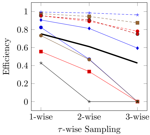
(c) Efficiency of Samples
