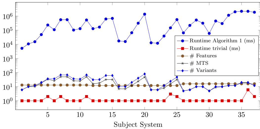
Figure 13: Results for the Synthetic Studies with Logarithmic y-Axis
