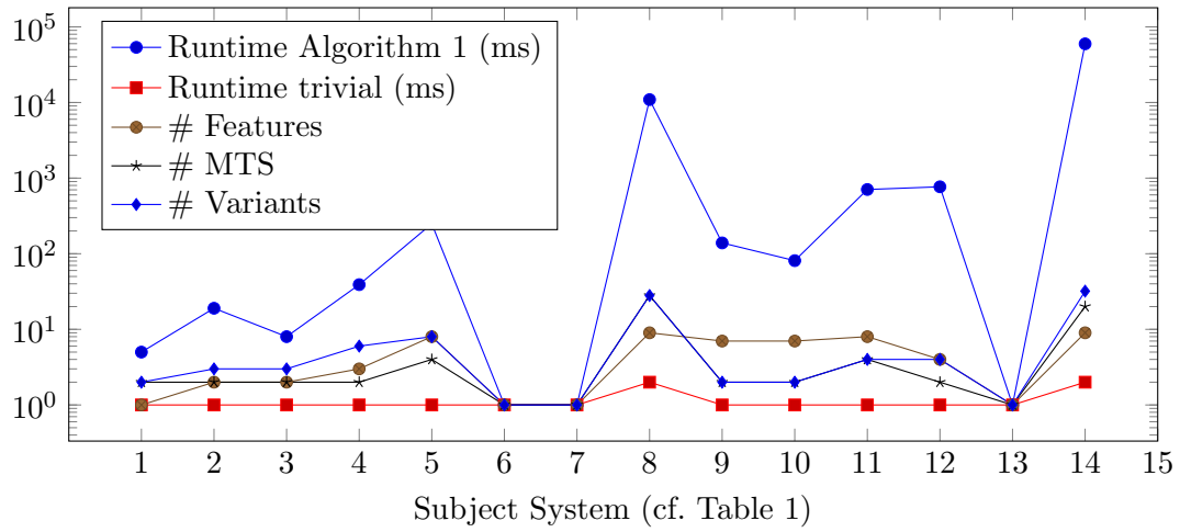
Figure 12: Results for the Real-Word Case Studies (cf. Table 1) with Logarithmic y-Axis
