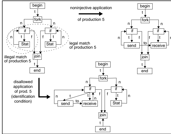
Figure 6: Noninjective matches and the identification condition
